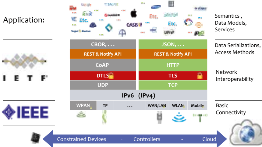
Fig 2: Typical IoT Technology Stacks
