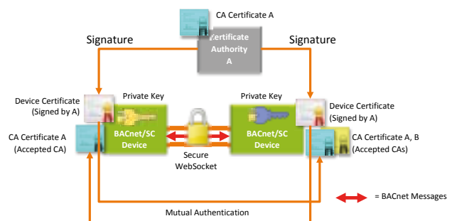
Figure 2: BACnet/SC Device Configuration for Secure WebSockets © BACnet International
